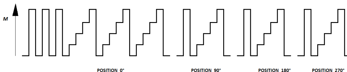
Figure 1. Measured torque measurement sequence diagram.
