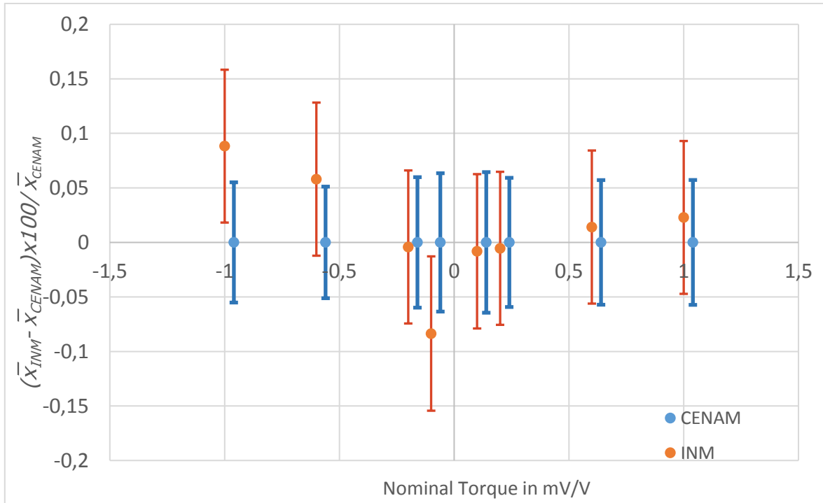
Figure 2. Comparison between the results obtained by the laboratories. The average error and uncertainty is included.
